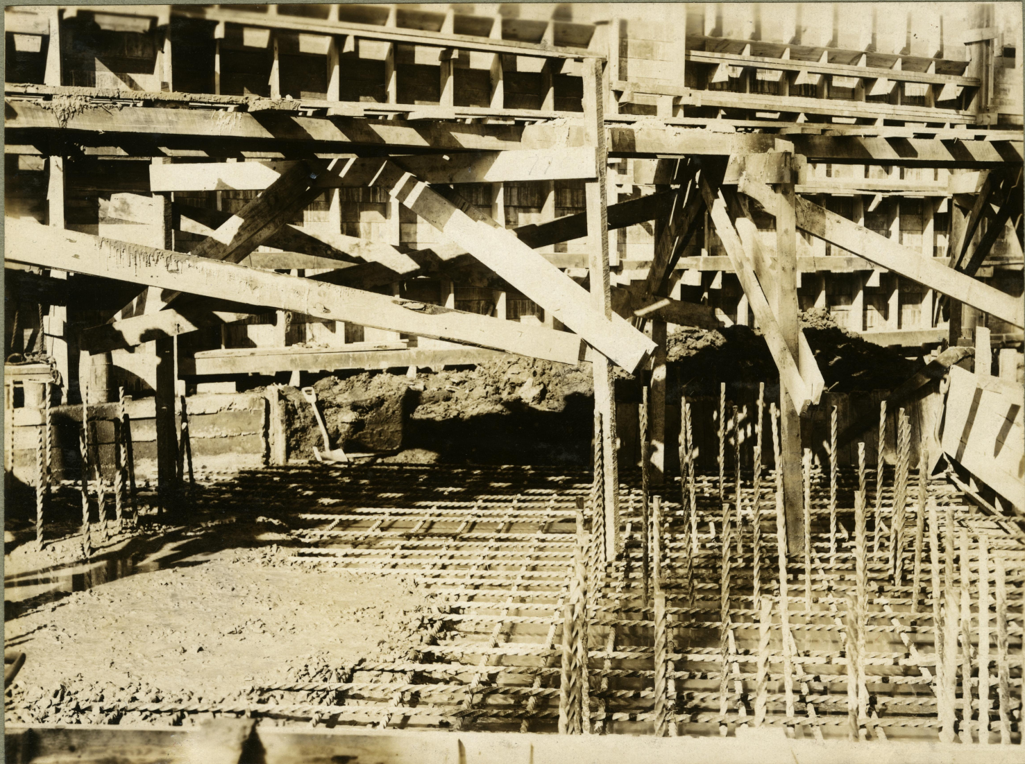
Reinforcement in Foundation ~ Nov. 6, 1914
