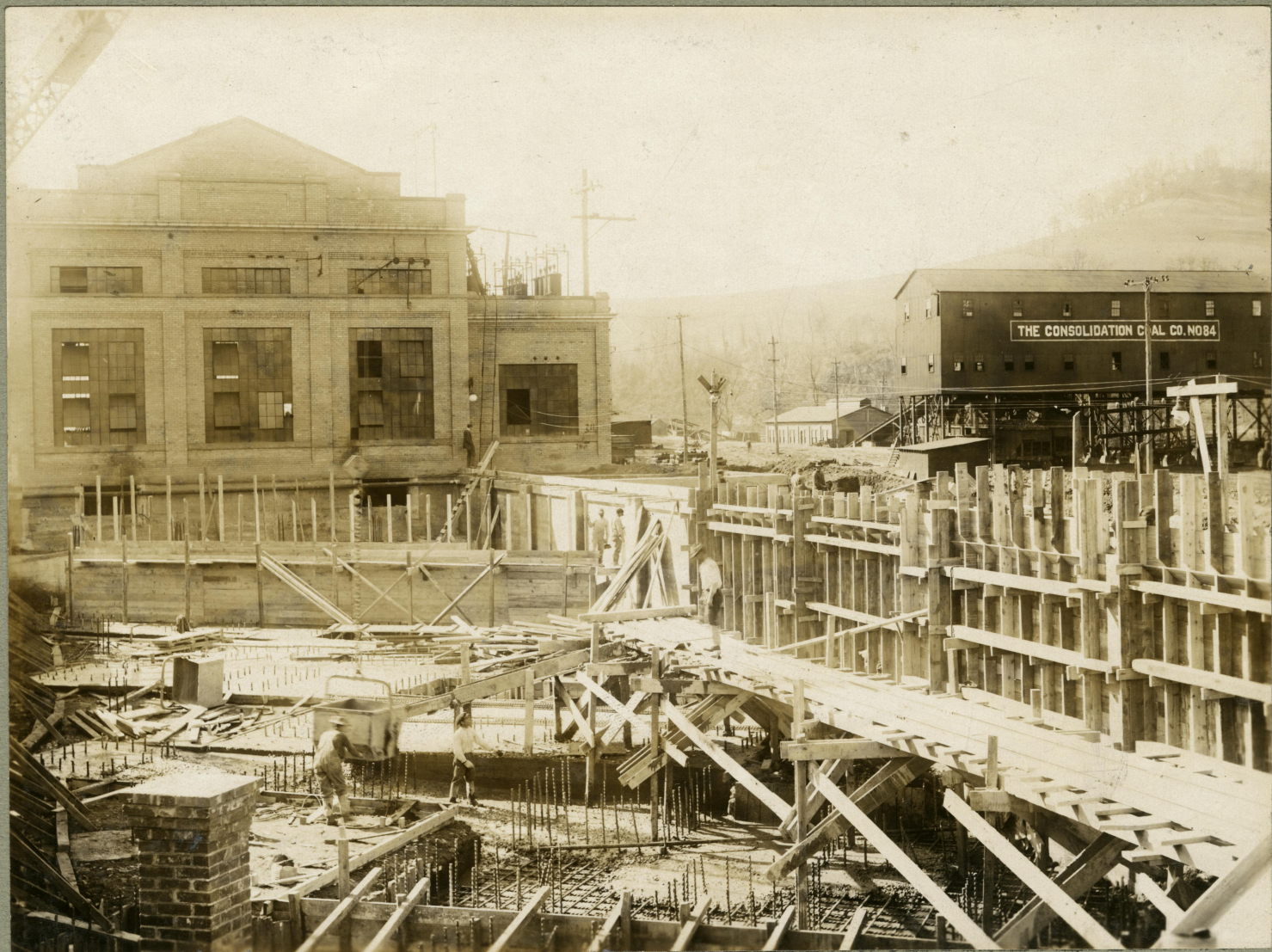
Concrete Foundation ~ Nov. 6, 1914
