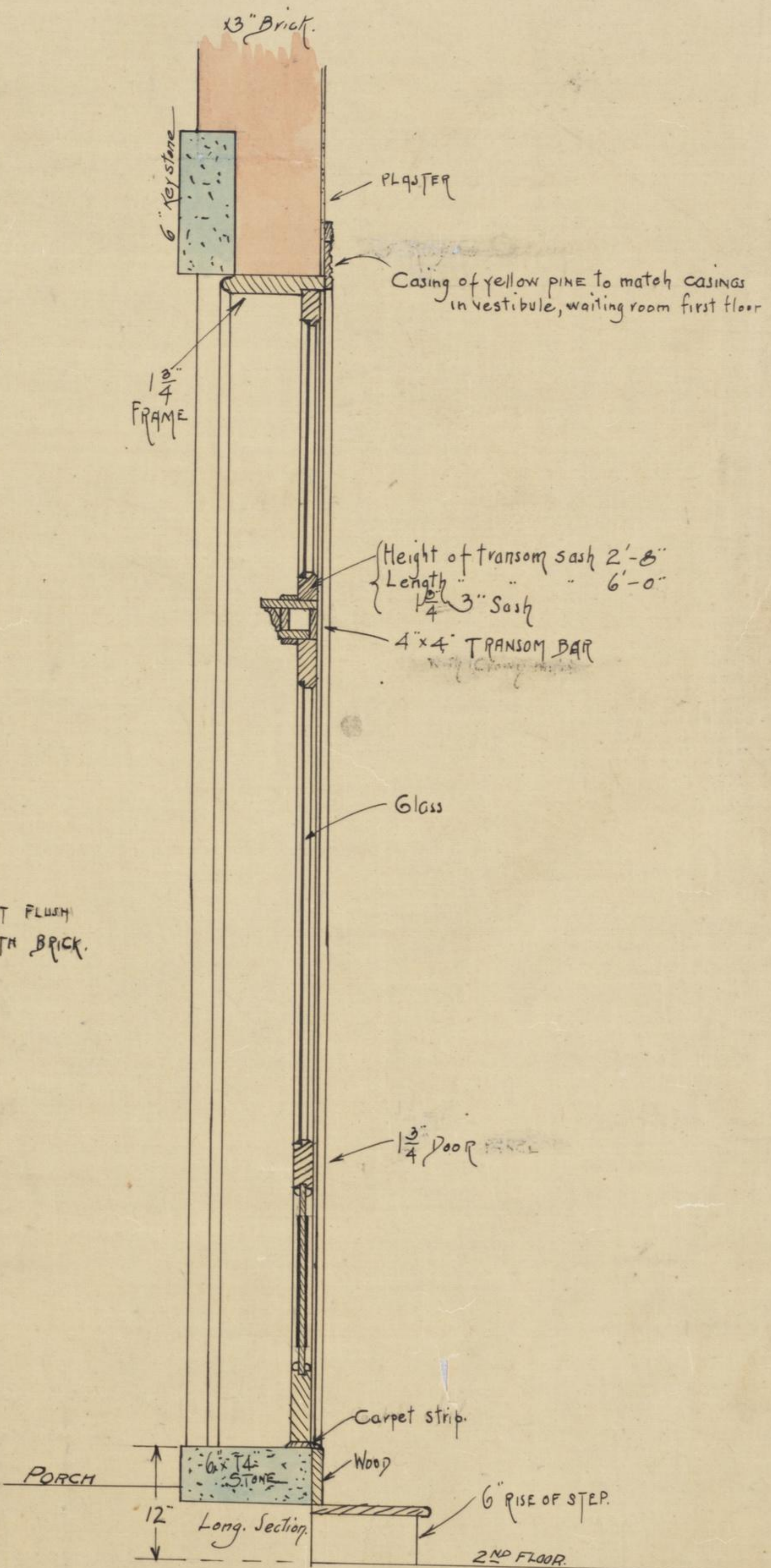
DETAIL OF DOUBLE DOORS ON SECOND FLOOR, FRONT ELEVATION OF GOOD SAMARITAN HOSPITAL
