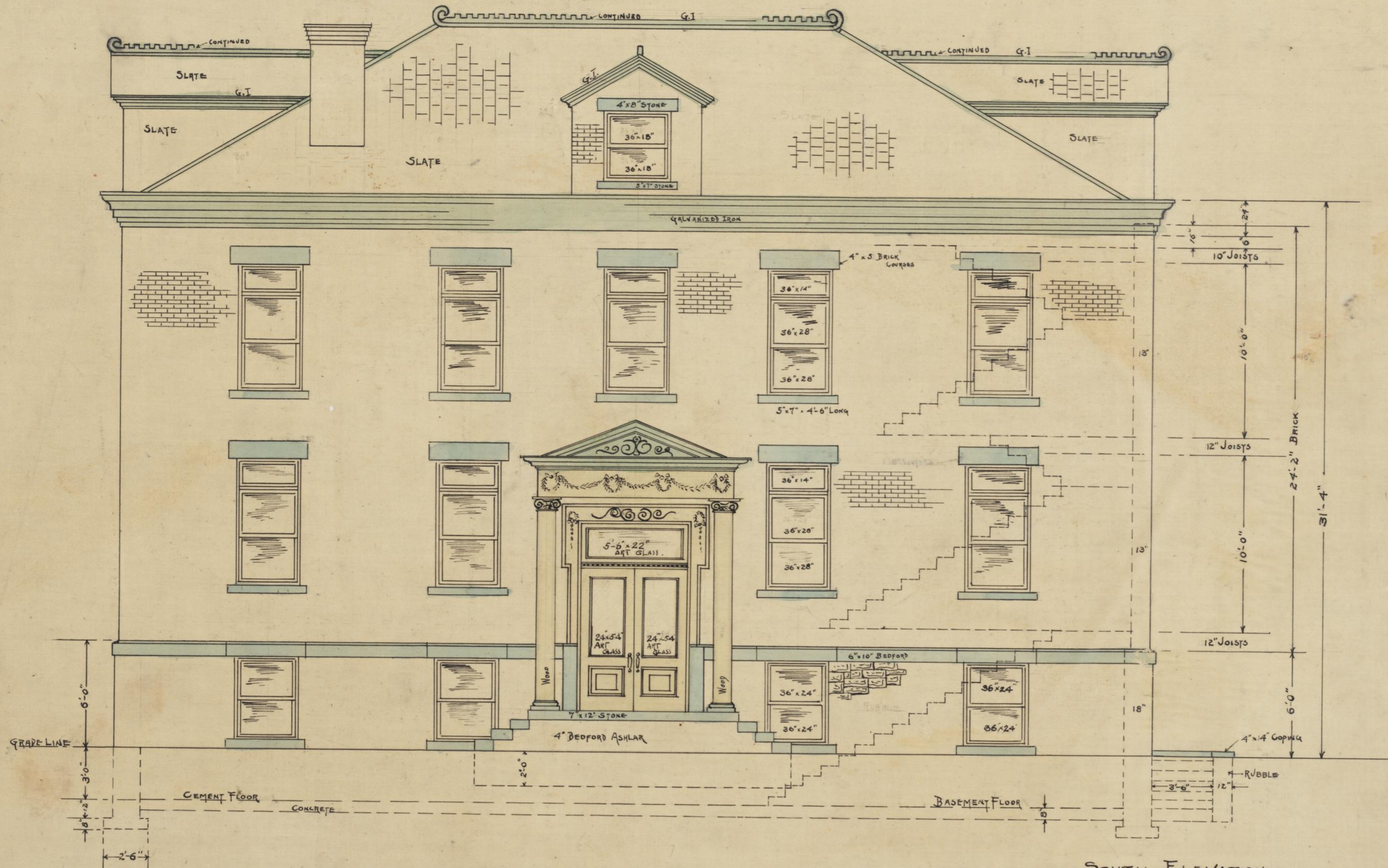
SOUTH ELEVATION BUILDING FOR COLORED PEOPLE GOOD SAMARITAN HOSPITAL LEXINGTON KY. ANDERSON & FAIG ARCHITECTS & ENGINEERS AUG. '06. SCALE: 1/4" = 1 FT.
