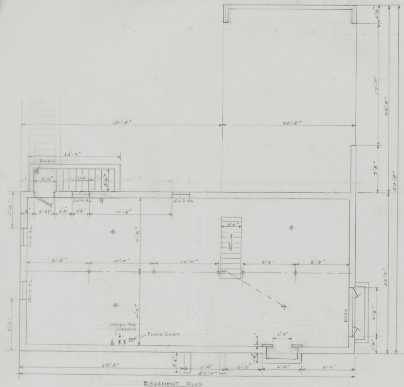
BASEMENT PLAN
