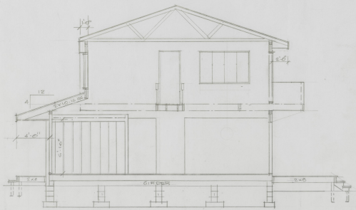
SECTION 1/4" = 1'-0"
