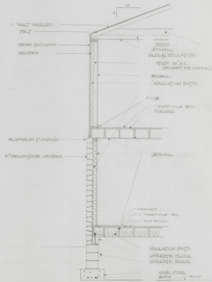
WALL SECTION 1/2" = 1'-0"
