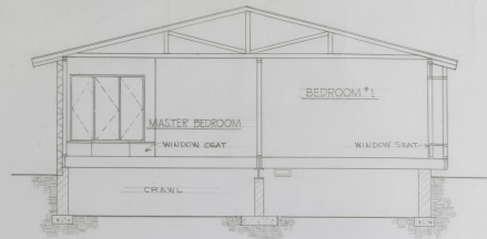
SECTION A-A 1/4" = 1'-0"
