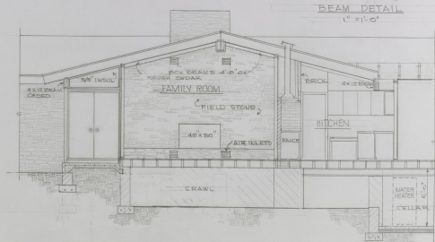
SECTION B-B 1/4" = 1'-0"
