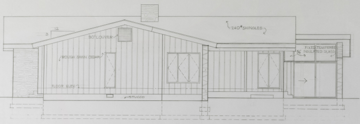
LEFT ELEVATION 1/4" = 1'-0"
