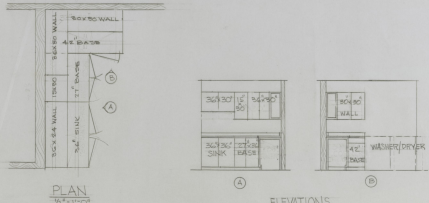
ELEVATIONS 1/4" = 1'-0"
