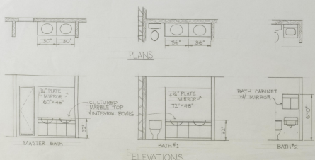
ELEVATIONS
