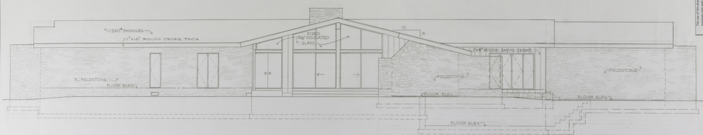
FRONT ELEVATION 1/4" = 1'-0"
