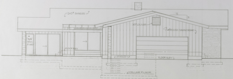
RIGHT ELEVATION 1/4" = 1'-0"
