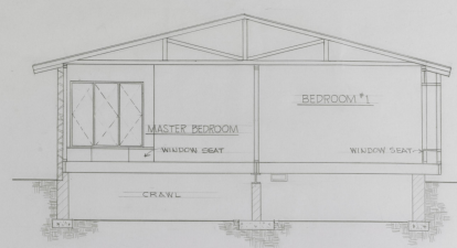
SECTION A-A 1/4" = 1'-0"
