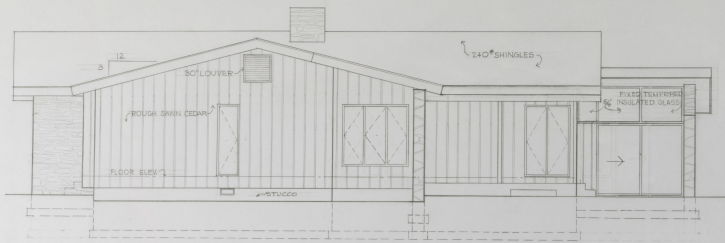
LEFT ELEVATION 1/4" = 1'-0"
