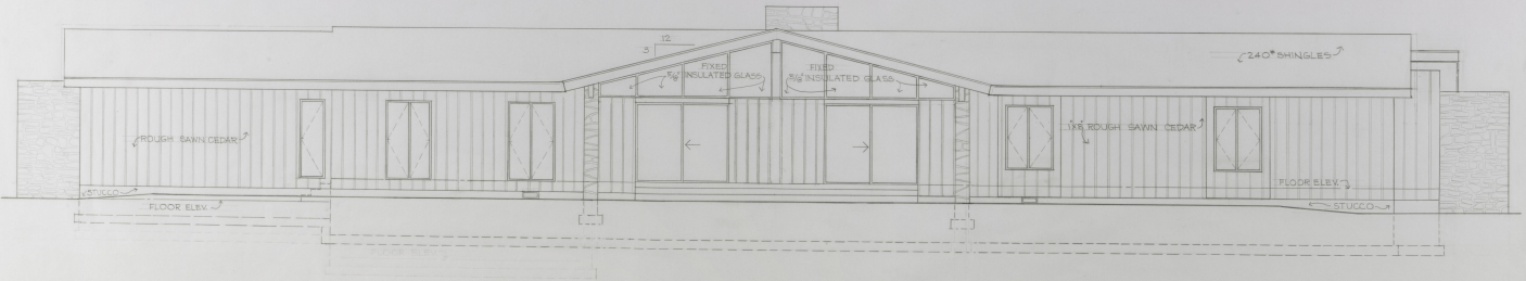
REAR ELEVATION 1/4" = 1'-0"
