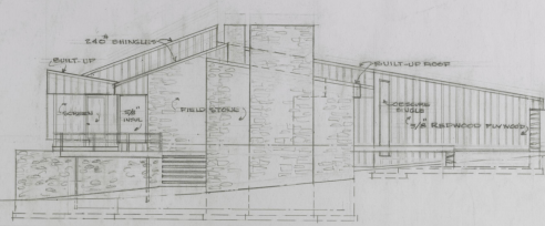
LEFT SIDE ELEVATION
