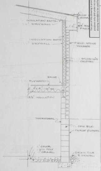
WALL SECTION 1/2" = 1'-0"
