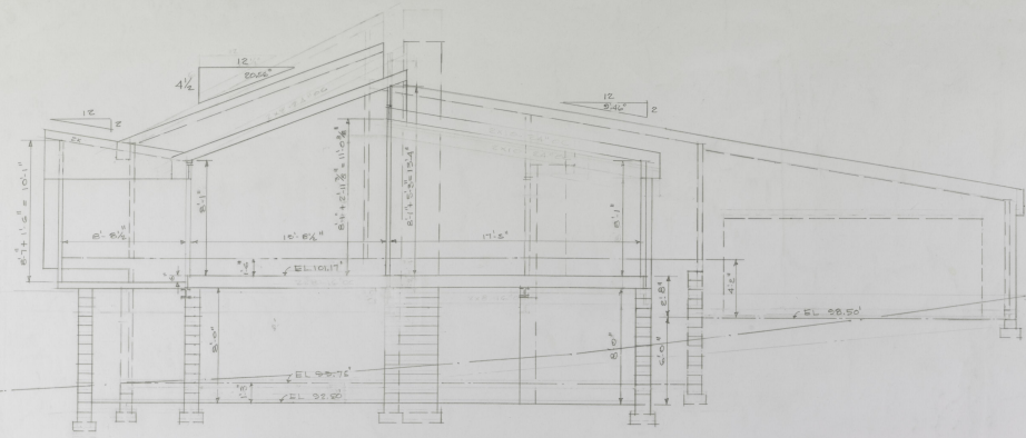
FRAMING SECTION - LIVING ROOM 1/4" = 1'-0"
