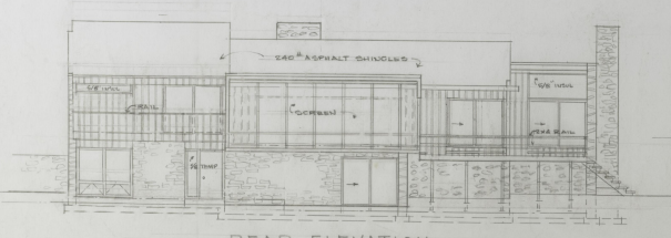
REAR ELEVATION
