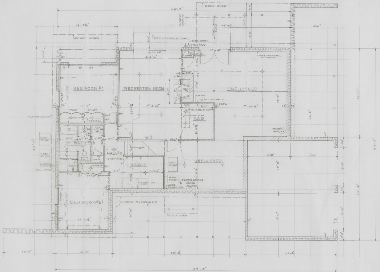
LOWER LEVEL PLAN 1/4" = 1'-0"
