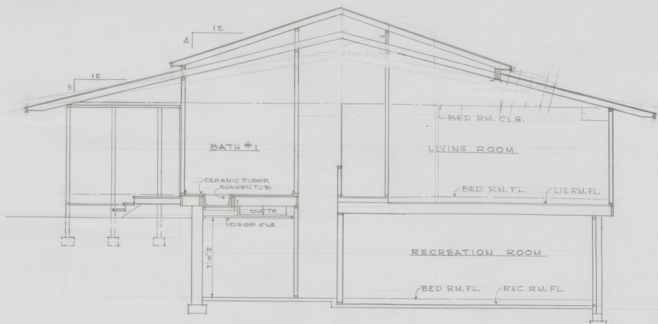
SECTION 1/4" = 1'-0"
