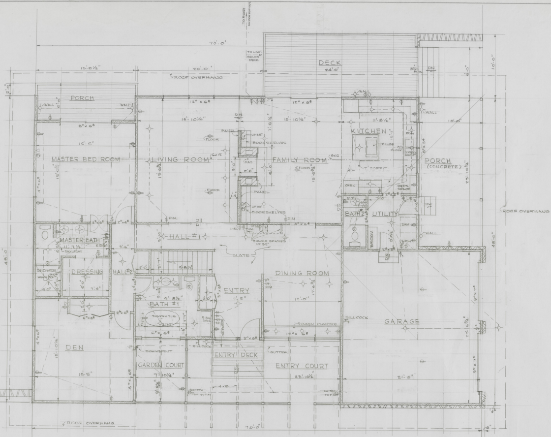
PLAN 1/4" = 1'-0"
