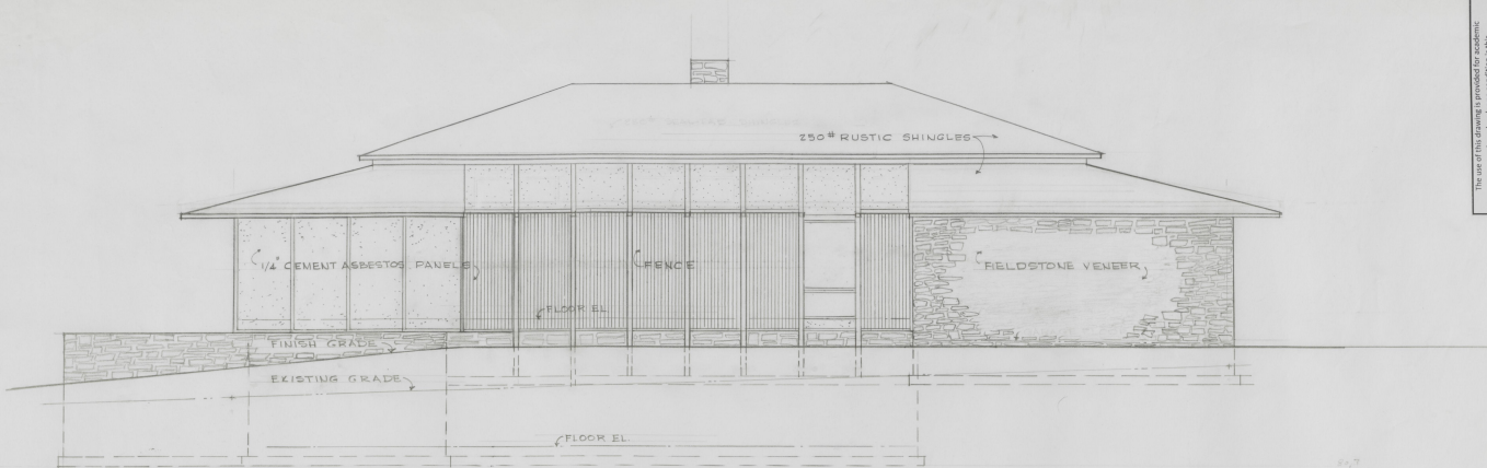
FRONT ELEVATION 1/4" = 1'-0"
