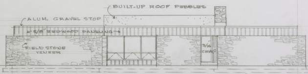
FRONT ELEVATION 1/8" = 1'-0"
