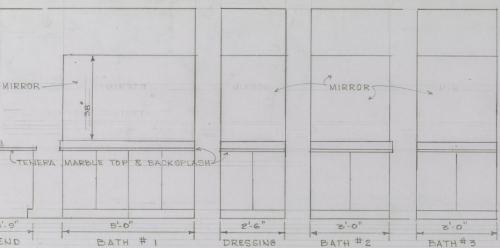
BATH VANITIES 1/2" = 1'-0"
