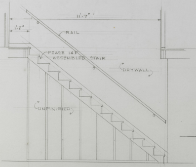
STAIR SECTION 1/2" = 1'-0"
