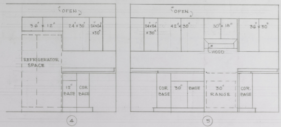
KITCHEN CABINET ELEVATIONS 1/2" = 1'-0"
