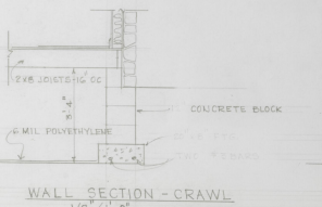
WALL SECTION-CRAWL 1/2" = 1'-0"
