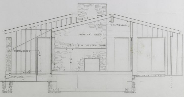
SECTION-FAMILY ROOM-GREENHOUSE 3/8" = 1'-0"
