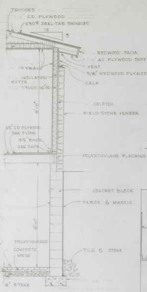
WALL SECTION-BASEMENT 1/2" = 1'-0"
