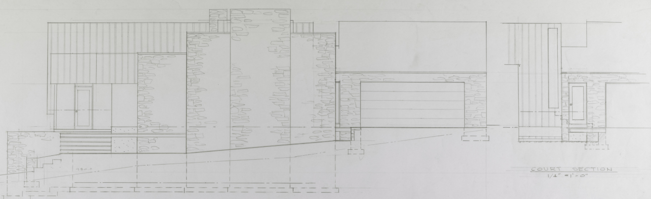
LEFT SIDE ELEVATION 1/4" = 1'-0"
