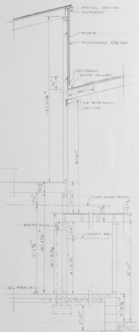
SECTION AA 1/2" = 1'-0"
