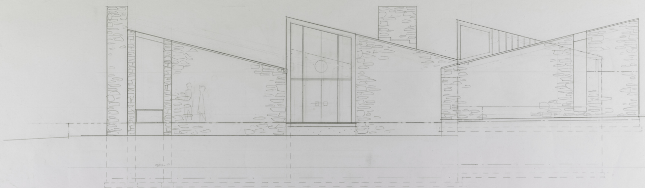
FRONT ELEVATION 1/4" = 1'-0"
