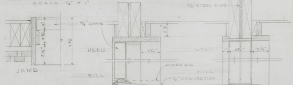
OUTSIDE DOOR DETAIL
