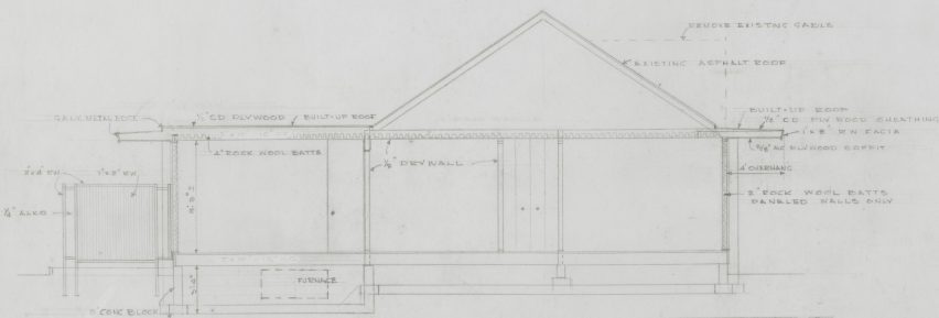
SECTION
