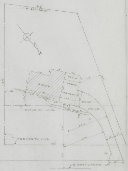
PLOT PLAN SCALE: 20' = 1"
