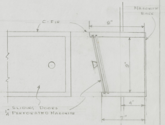
BATHROOM STORAGE CAB. DETAIL SCALE 3/4" = 1'-0"
