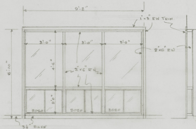
DETAIL L.P. & KITCH. WINDOW SCALE 1/2" = 1'-0"
