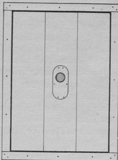
Fig. 3—Bee-escape and board.
