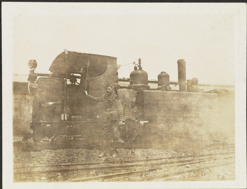
Narrow Gauge - Steam Locomotive, Gauge 23"
