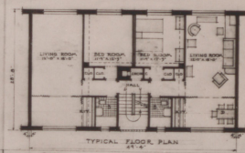
TYPICAL MULTI-FAMILY BUILDING GREENBELT MARYLAND
