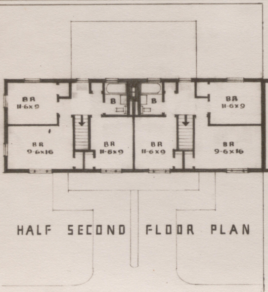
° TYPICAL GROUP HOUSE ° GREENDALE ° ° ° ° ° WISCONSIN
