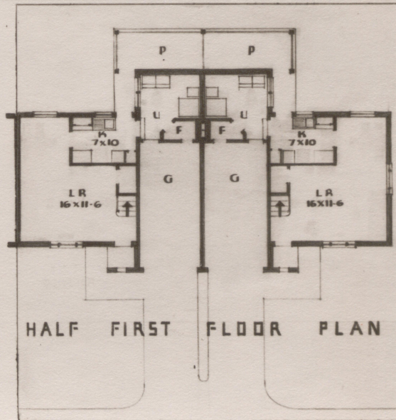
° TYPICAL GROUP HOUSE ° GREENDALE ° ° ° ° ° WISCONSIN
