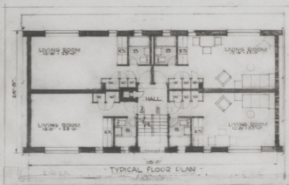
TYPICAL MULTI-FAMILY BUILDING GREENBELT MARYLAND
