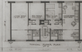
TYPICAL MULTI-FAMILY BUILDING GREENBELT MARYLAND
